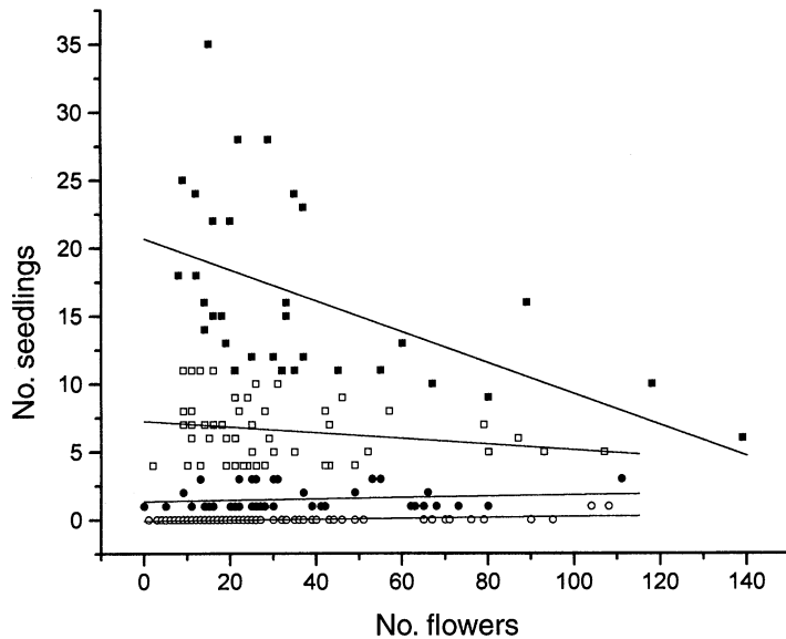
FIG. 6. Two-cycle partitioned regression of seedlings vs. flowers for the Washington Gulch grid of 256 2 \times 2 m quadrats. First, a major-axis regression line through all the points was used to partition the data into upper and lower subsets. Then each subset was similarly partitioned, yielding four subsubsets denoted here by different symbols. Major axes are shown for each of the subsubsets. One outlier, evident in Fig. 5, has been removed. Points are not jittered, so some near the origin are obscured.
