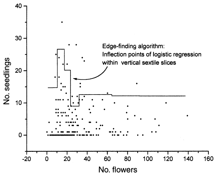
FIG. 7. Logistic slicing of the seedlings vs. flowers relationship. The lengths of the horizontal line segments indicate the widths of the six vertical slices, and their vertical position indicates the height of the inflection points that approximate the edge of the point cloud.
